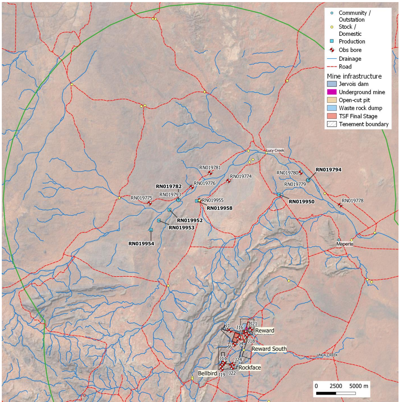
Figure 6-1 Locations of observation bores around the process water supply borefield (bold labels).
